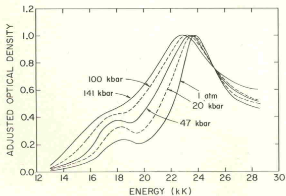
FIG. 3. Optical absorption spectra of imidazole photohemichrome vs pressure.
