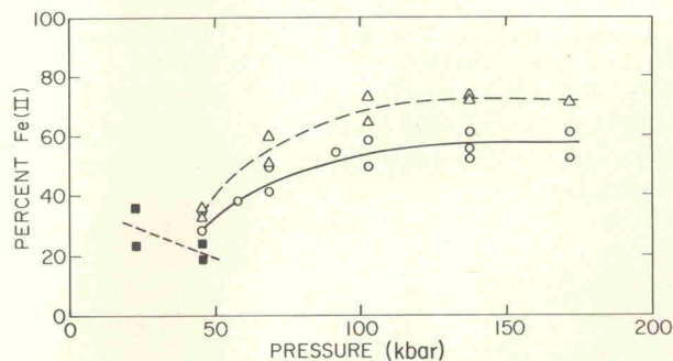
FIG. 6. Conversion of ferric to ferrous iron vs pressure for imidazole protohemichrome. O, Fe(II) [I.S.] 23°C; \Delta , Fe(II) [I.S.] 110°C; \blacksquare , Fe(II) [L.S.] 110°C.
